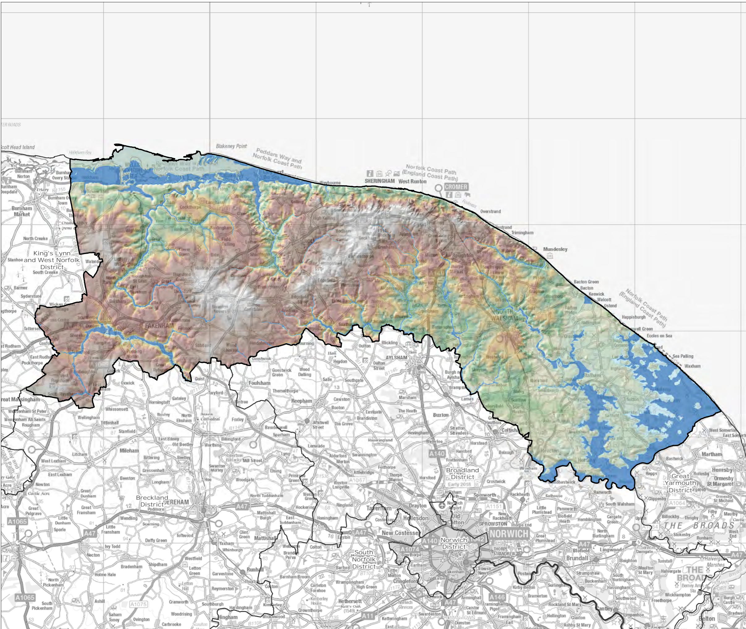
Figure 3.3: Topography & Drainage
