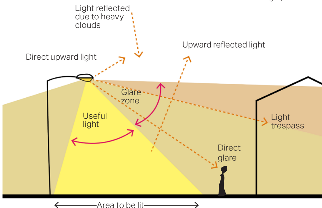
Figure 47: Diagram to illustrate the different components of light pollution and what 'good' lighting means.
