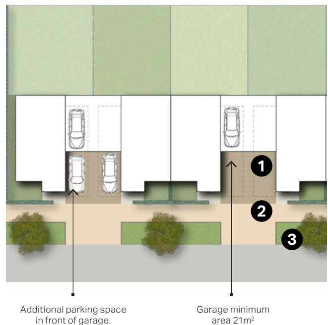
Figure 32: Local example of on-plot garage typology.
