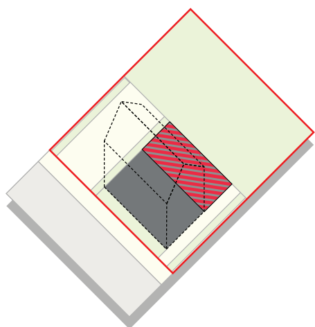
Figure 62: Diagram illustrating the basic principle about 50% coverage of the plot area for both the main building and annex.
