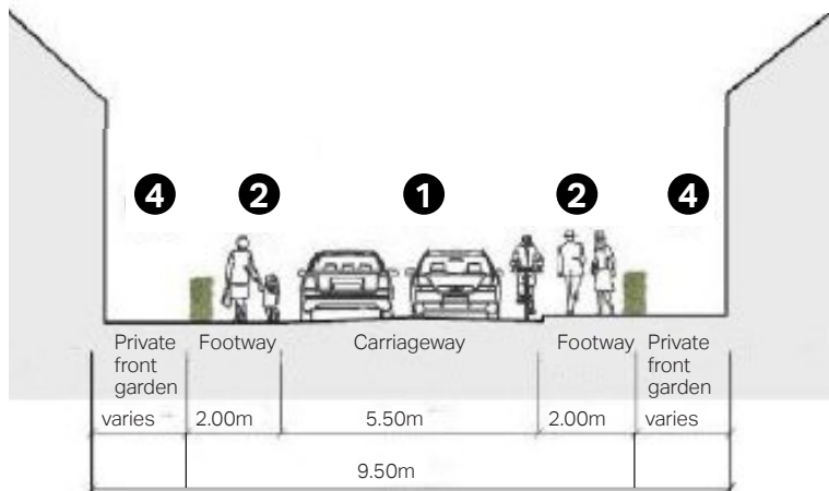
Figure 26: Section showing indicative dimensions for residential streets.
