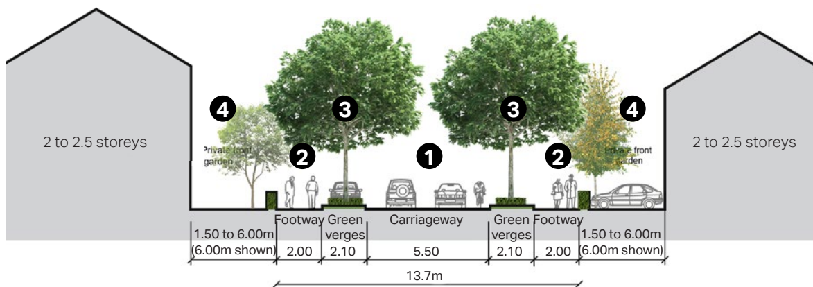
Figure 25: Section showing indicative dimensions for residential streets with green verges.
