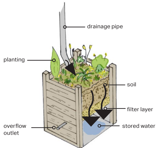
Figure 94: Diagram illustrating the functioning of a stormwater planter.
