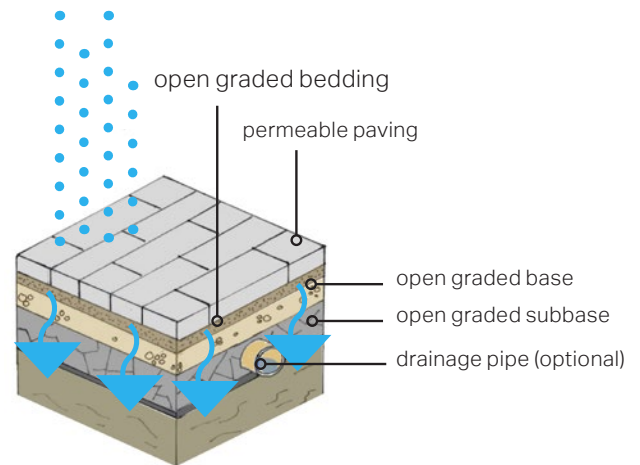
Figure 97: Diagram illustrating the functioning of a soak away.
