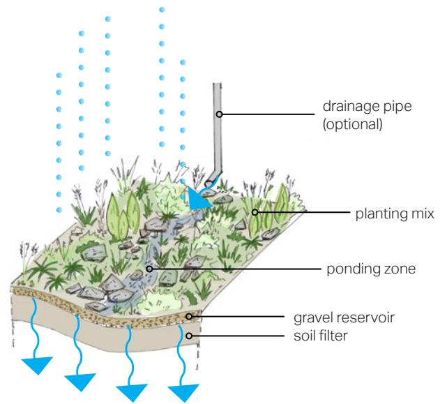
Figure 96: Diagram illustrating the functioning of a rain garden.
