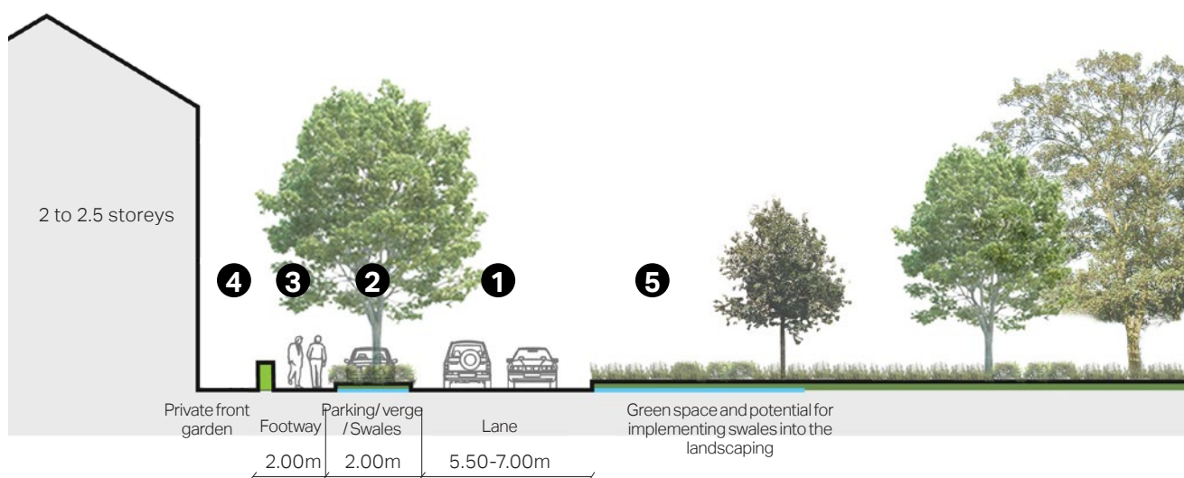
Figure 24: Section showing indicative dimensions for main entrances.
