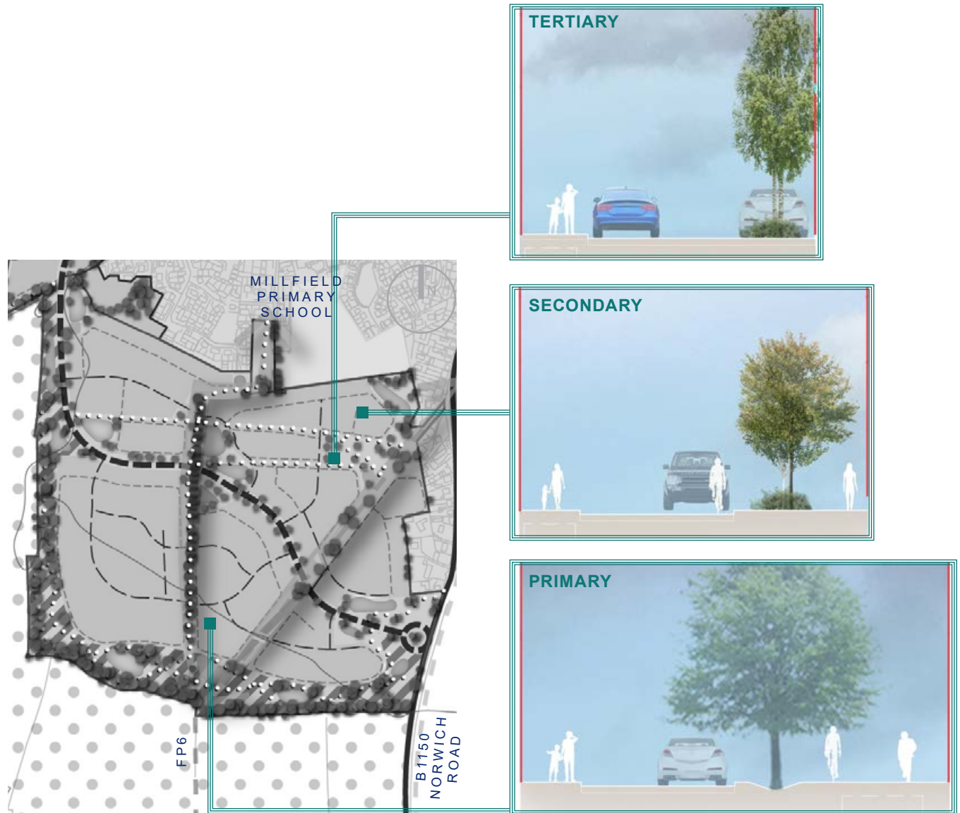
Figure 108; Typical road sections
